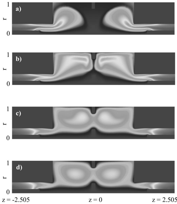
FIG. 3. Evolution of magnetic flux from TRIM simulation. (a) Formation t = -2.73 \mu s , (b) merging t = 0 \mu s , (c) relaxation t = 13.5 \mu s , (d) equilibrium t = 23.4 \mu s . t = 0 is defined as the time of maximum magnetic energy in the reconnection zone (see Fig. 5). Dimensions are normalized to the radius of the flux conserver.
