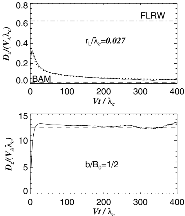
Figure 1. Results of a test particle simulation with r_L/\lambda_c = 0.027 and \delta b/B_0 = 0.5 . (Bottom panel) Solid line is running parallel diffusion coefficient vs. time. For reference, dashed line is approximate quasilinear theory result. (Top panel) Solid line is running perpendicular diffusion coefficient. Dotted line corresponds to subdiffusion. FLRW and BAM theoretical results (see text) are also shown.
