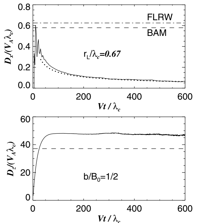
Figure 2. Results of another test particle simulation with r_L/\lambda_c = 0.67 , and \delta b/B_0 = 0.5 in same format as Figure 1. (Bottom panel) Running parallel diffusion coefficient vs. time. (Top panel) Running perpendicular diffusion coefficient.
