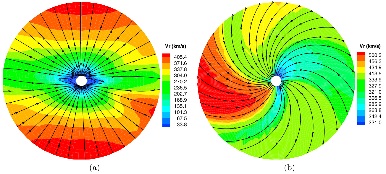
Figure 2. Magnetic field and radial speed for the steady state solar wind solution. (a) Solar coronal solution at \phi = 180^\circ – 0^\circ from 1R_s to 15R_s and (b) inner heliosphere solution in the solar equatorial plane from 15R_s to 215R_s . The color contours represent the radial speed and streamlines denote the magnetic field lines.
