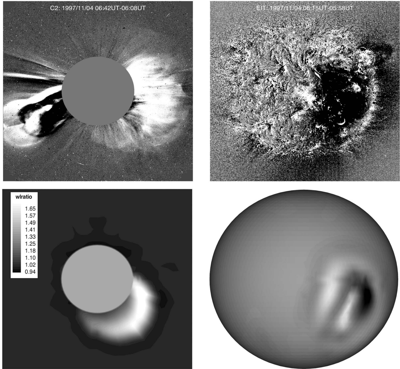
Figure 4. (top) C2 and EIT difference images. (bottom) Synthetic white light running ratio image corresponding to C2 field-of-view (left), numerically simulated density-enhancement image on the solar disk (right).
